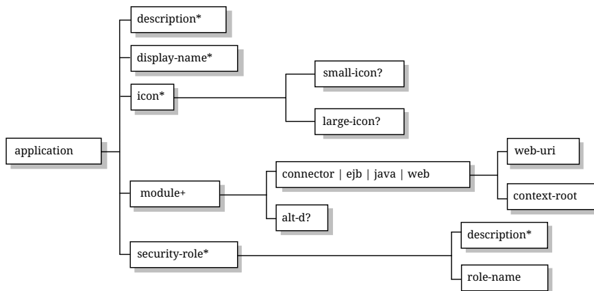
Figure 19. J2EE 1.4 Application XML Schema Structure
