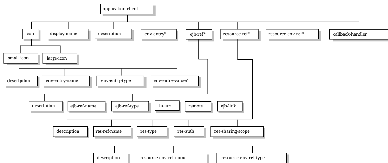
Figure 22. J2EE:1.3 application-client XML DTD Structure
