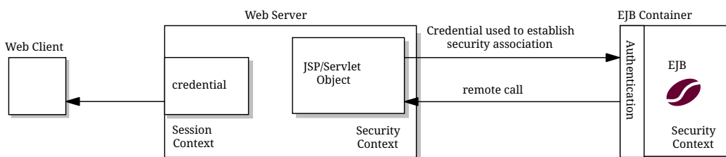
Figure 7. Invoking an Enterprise Bean Business Method
