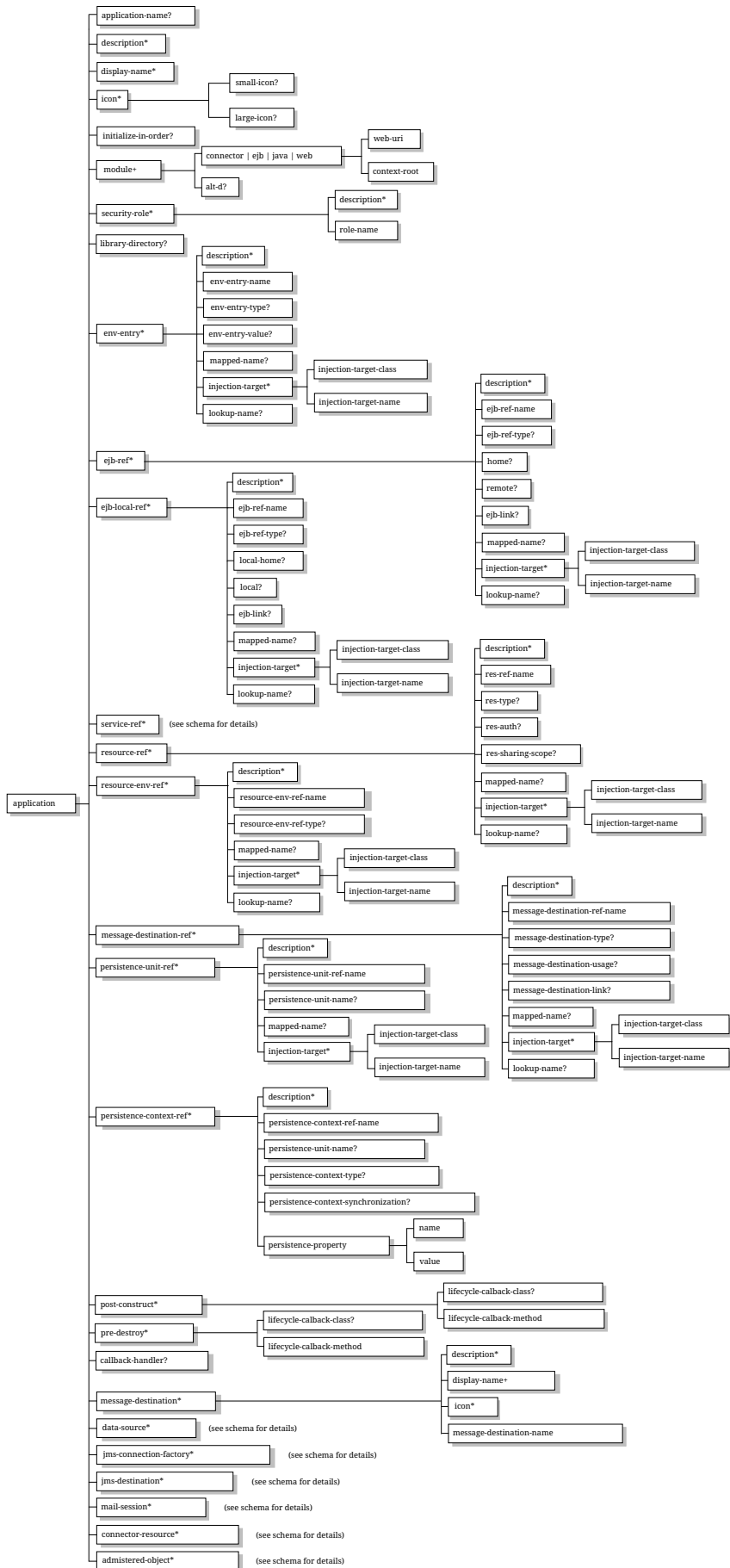
Figure 11. Jakarta EE Application XML Schema Structure
