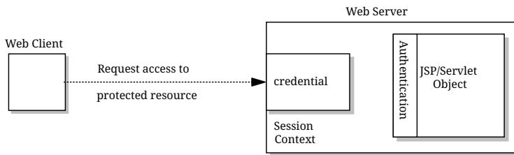
Figure 5. URL Authorization
