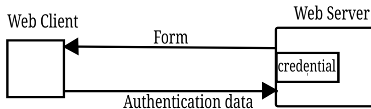
Figure 4. Initial Authentication
