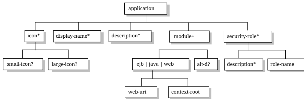
Figure 23. J2EE.1.2 application XML DTD Structure
