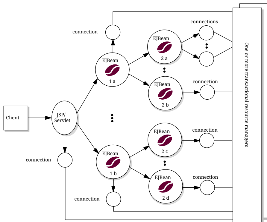
Figure 8. Servlets/Server Pages Accessing Enterprise Beans
