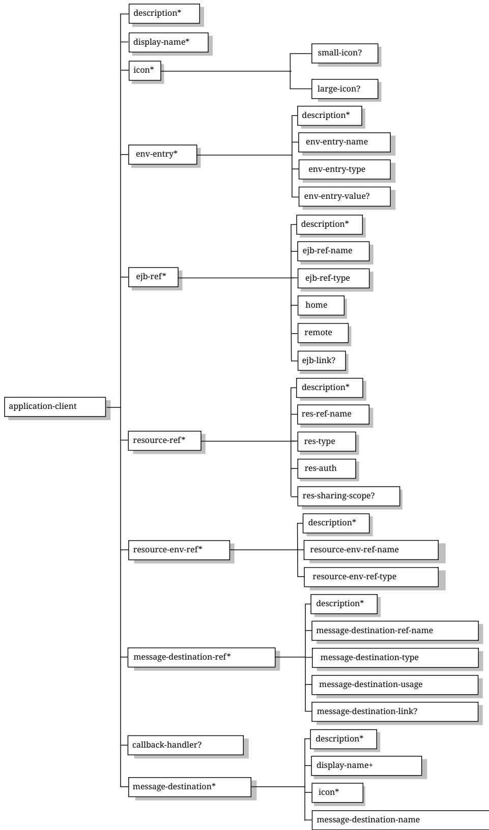
Figure 20. J2EE 1.4 Application Client XML Schema Structure
