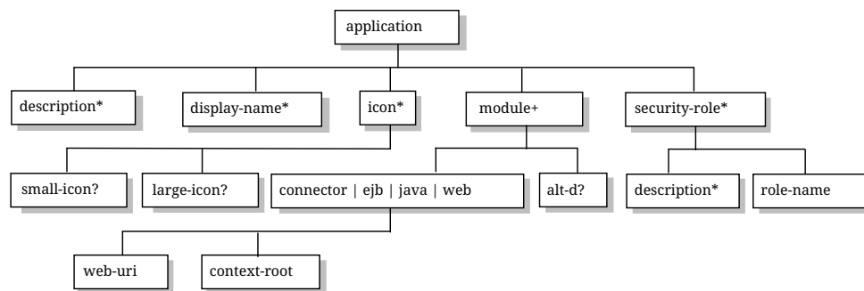
Figure 21. J2EE:1.3 application XML DTD Structure
