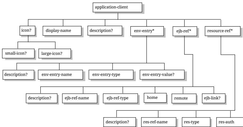
Figure 24. J2EE:1.2 application-client XML DTD Structure
